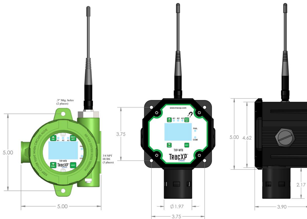
Figure 4-1 Mounting Diagrams (Aluminum and Polycarbonate Enclosures)
