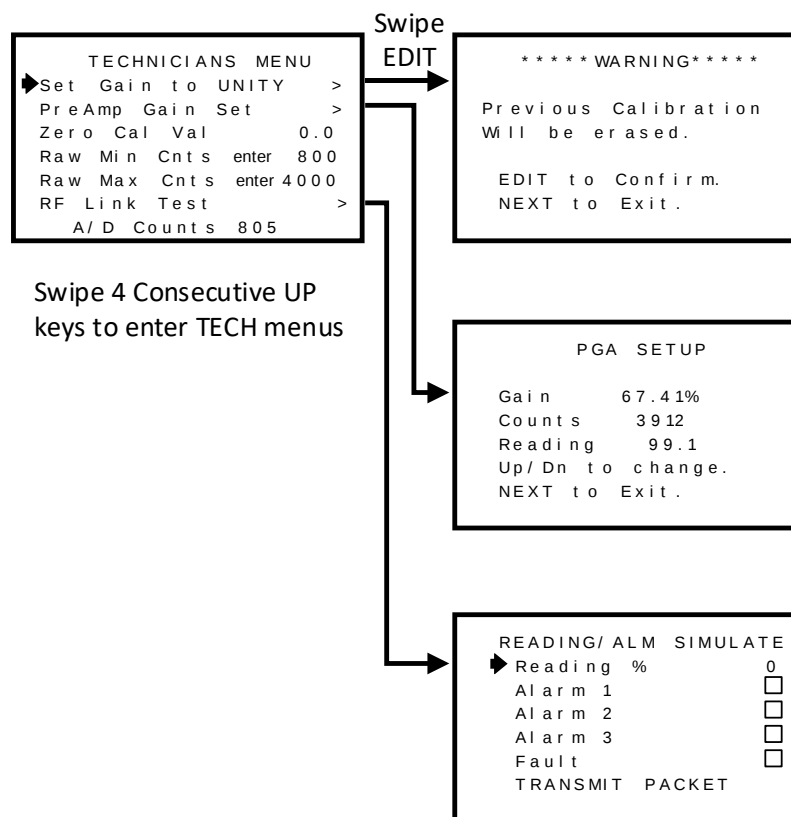
Figure 7-5 Technicians Menu Tree
