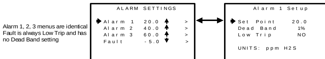
Figure 7-3 Alarm Settings Menus
