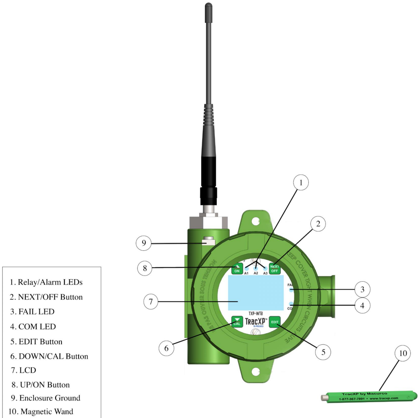
Figure 2-2 External System Diagram
