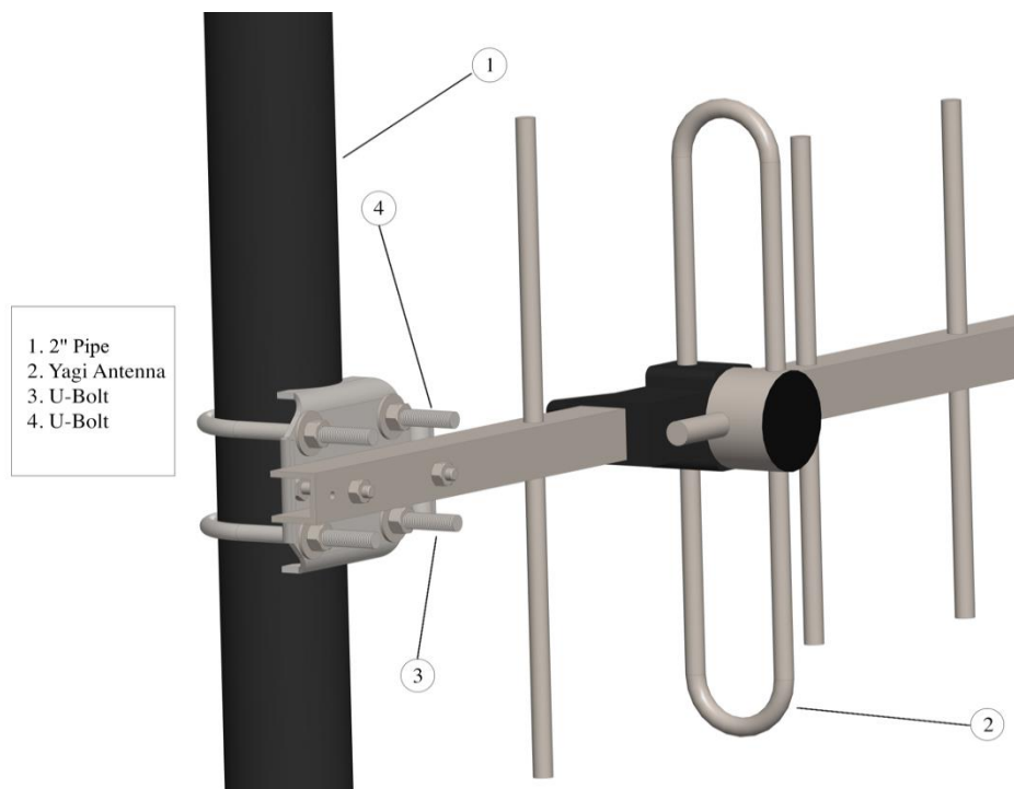
Figure 9-2 Yagi Antenna Installation Diagram
