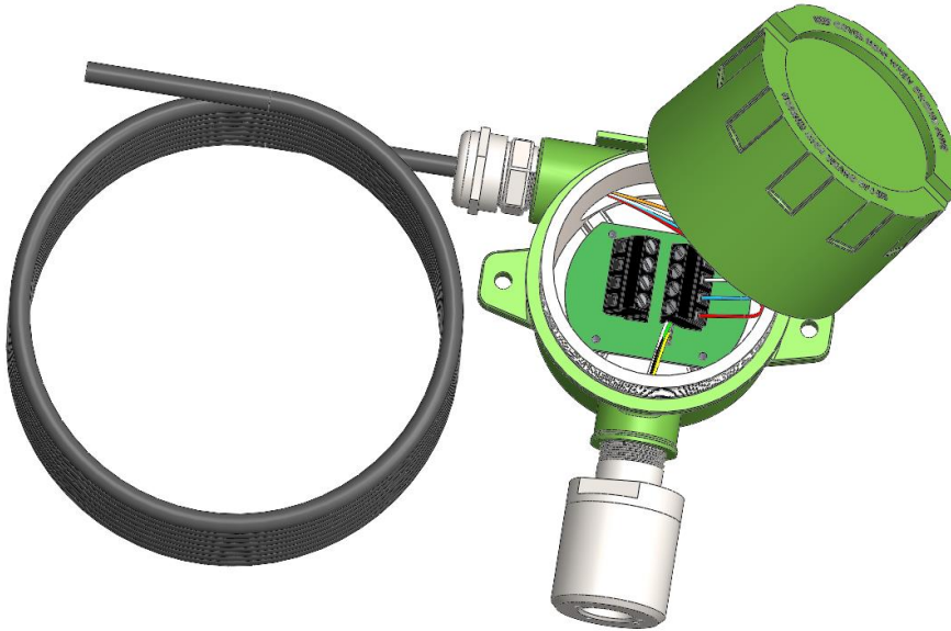
Figure 5-7 Sensor Separation Kit
