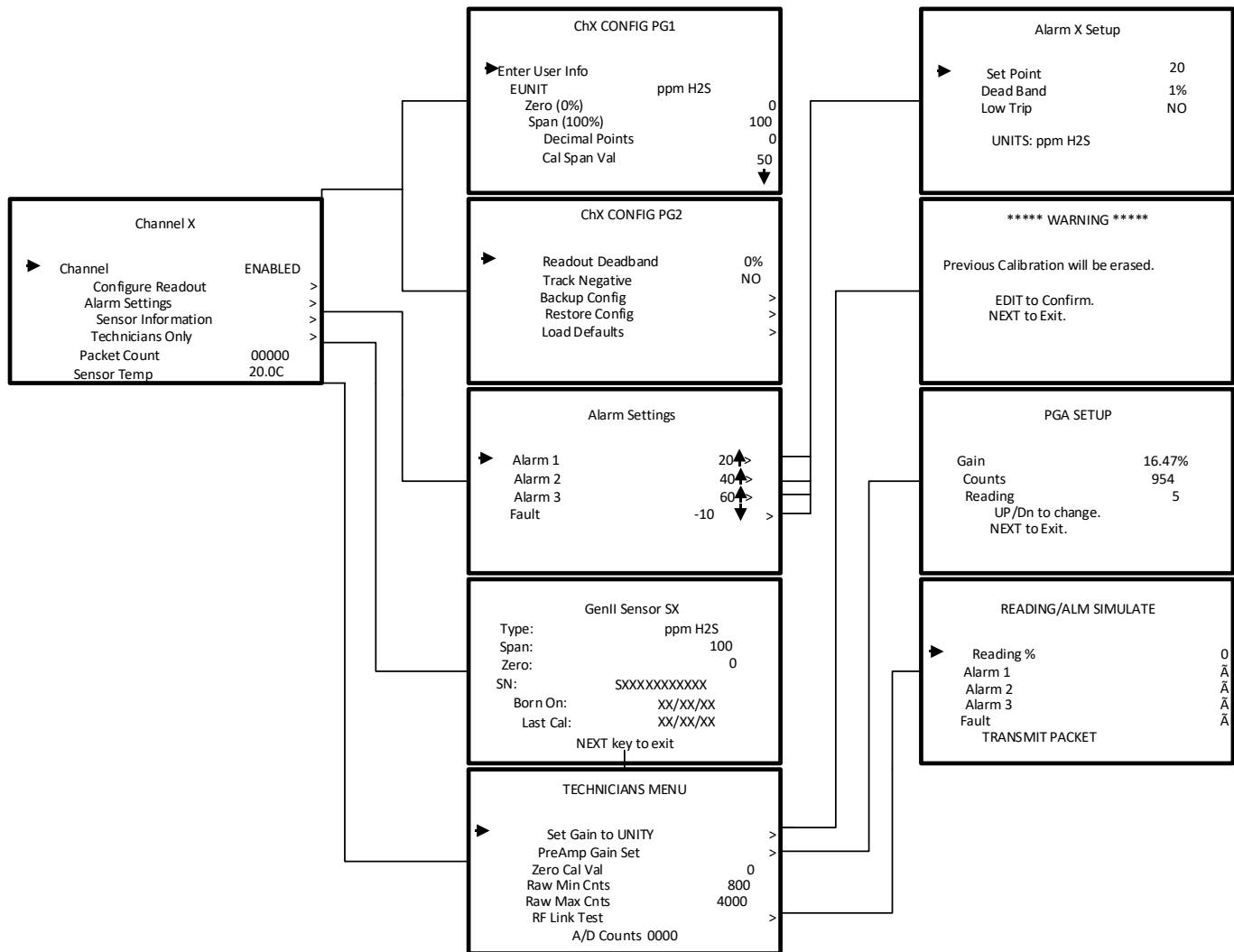
Figure 6-2 Channel Configuration Menu Tree
