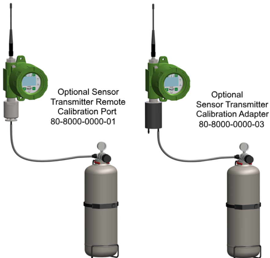
Figure 5-2 Calibration Gas Input
