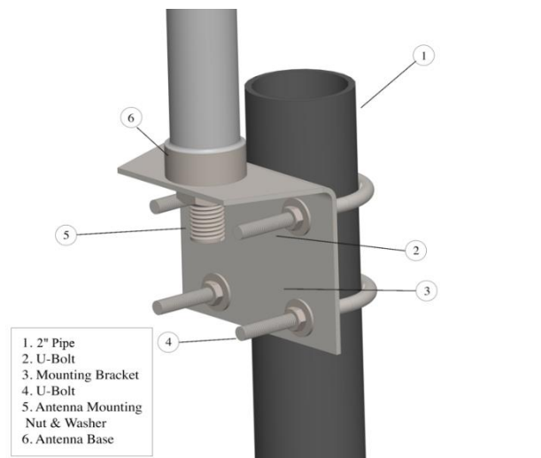
Figure 9-1 Dipole Antenna Installation Diagram
