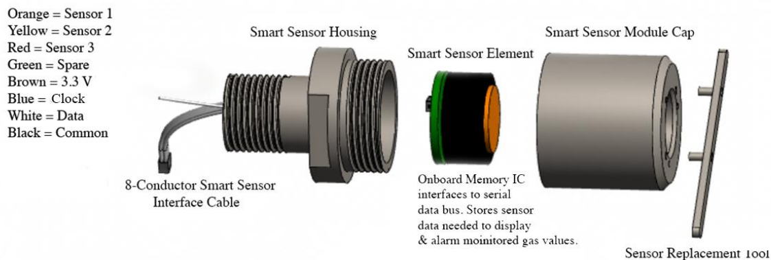
Figure 5-6 Smart Sensor Module 80-8000-00A0-10
