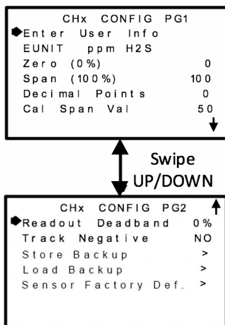
Figure 7-2 Configure Readout Setup Menus
