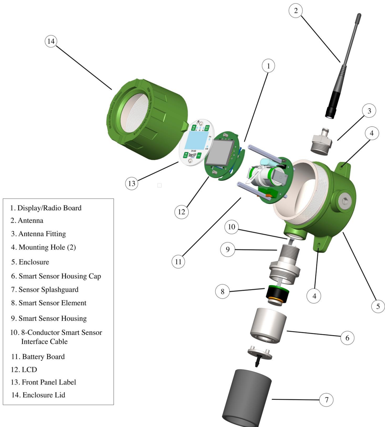
Figure 2-3 Transmitter Diagram
