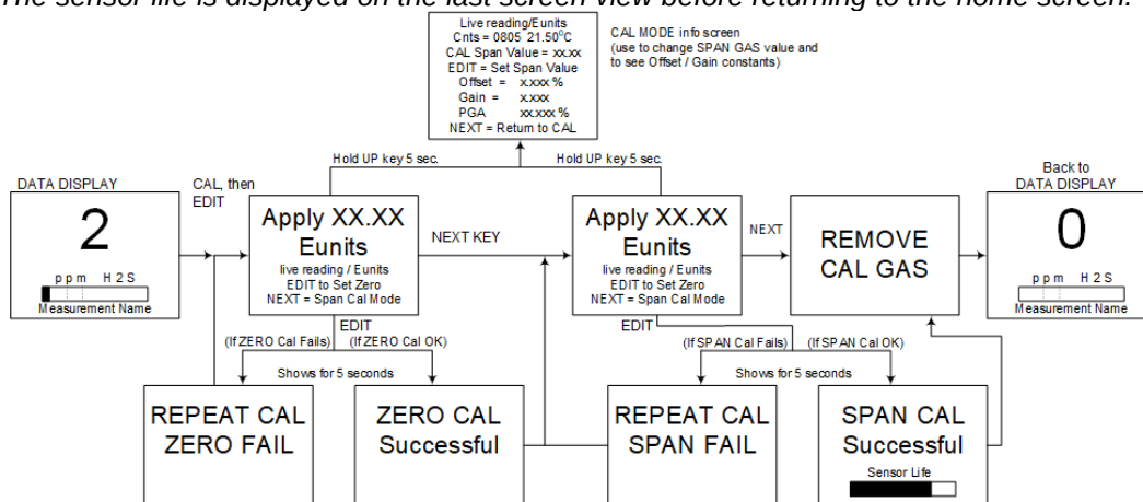
Figure 5-3 Cal-Mode Flow Chart and Menus
