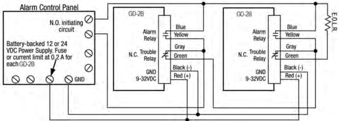
Figure 2 – Single Unit Wiring
