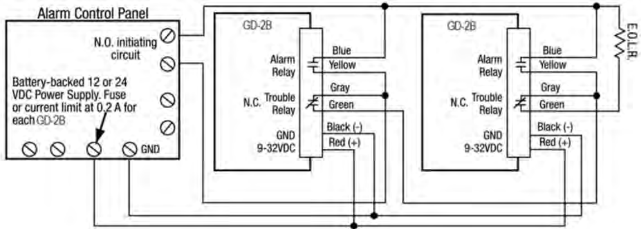
Figure 1 – Multiple Unit Wiring
