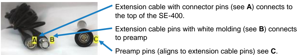
Figure 4-17: Example of extension cable and preamp
