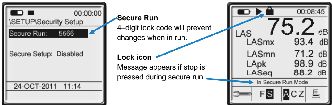
Figure 3-9: Secure run and measurement screen
