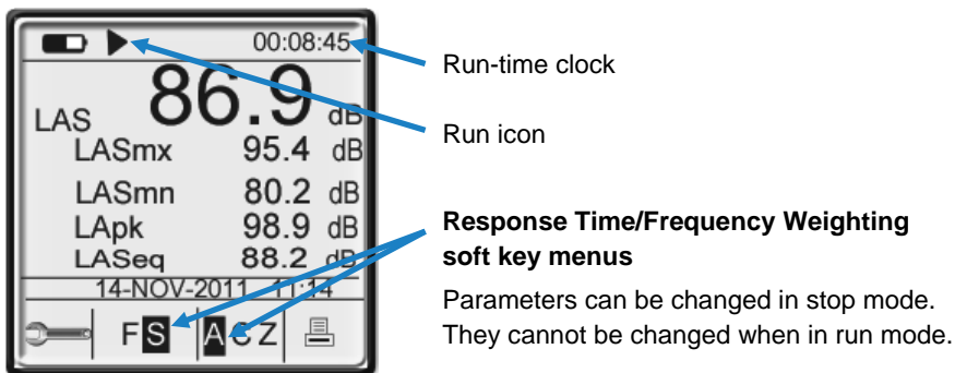
Figure 4-8: Main/multi-measurement screen in Run mode
