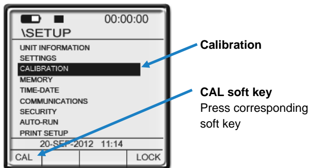
Figure 4-2: Calibration soft key selection
