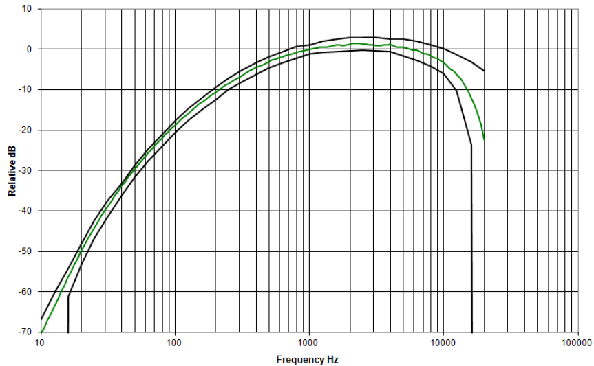
Figure C-5: A-weighting typical
