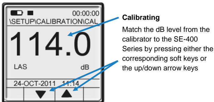
Figure 4-4: CAL screen
