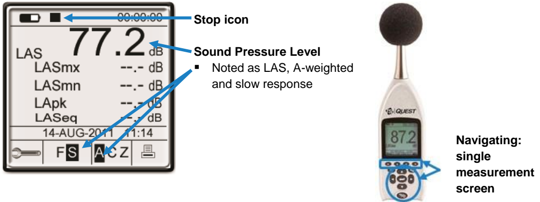
Figure 2-2: Measurement screen displaying multiple measurements
