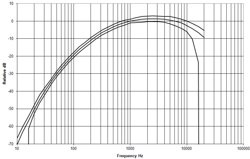
Figure C-2: A-weighting nominal
