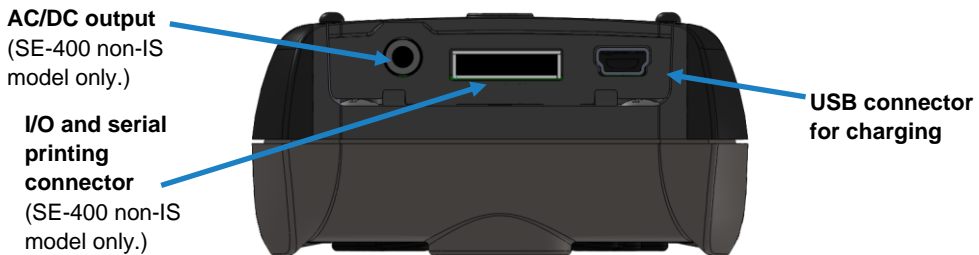
Figure 1-2: Connector and ports
