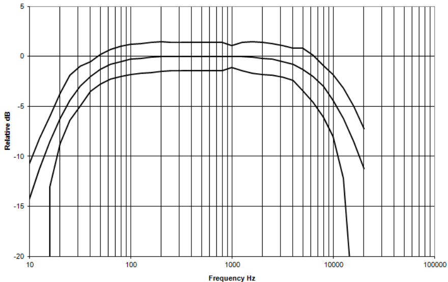
Figure C-3: C-Weighting nominal
