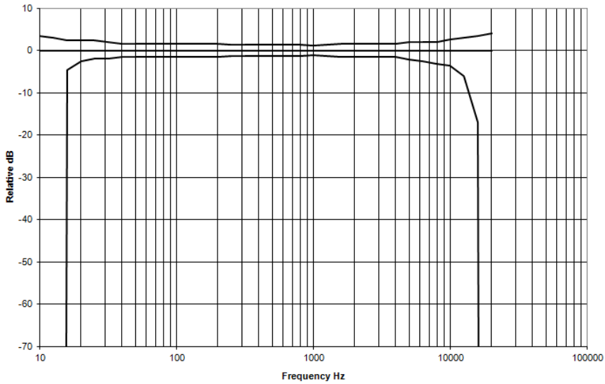
Figure C-4: Z-weighting nominal
