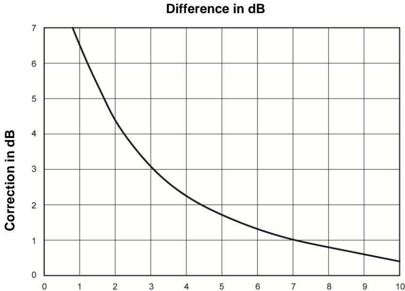
Figure C-1: Effects of background noise
