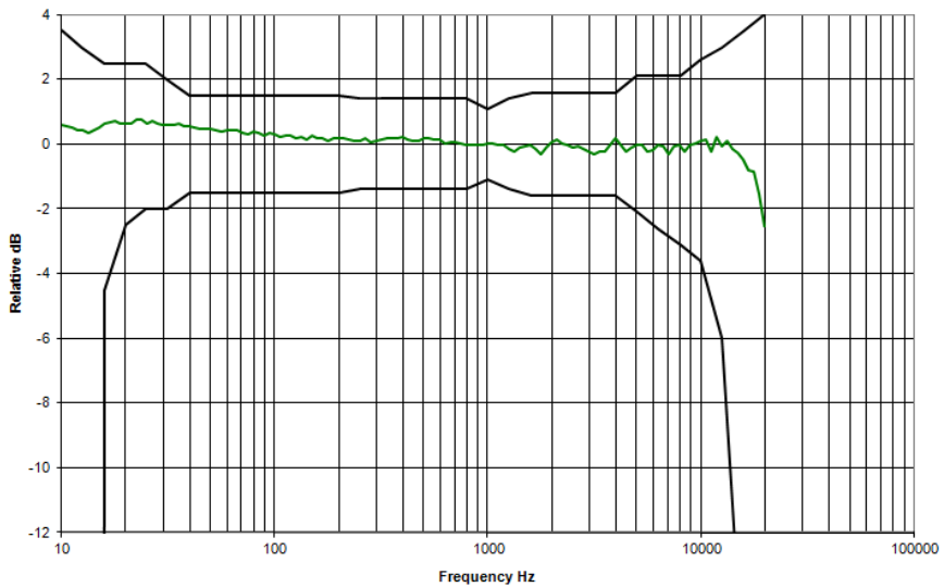
Figure C-7: Z-weighting typical
