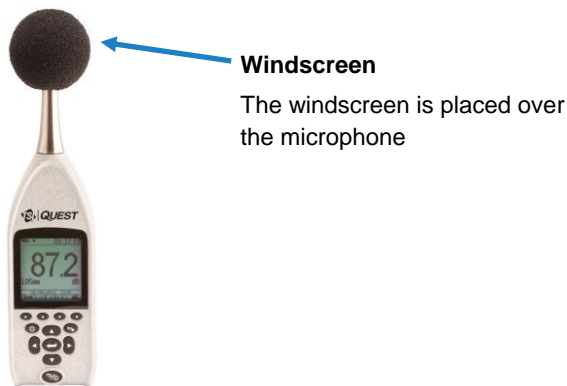
Figure 4-6: SE-400 Series with windscreen
