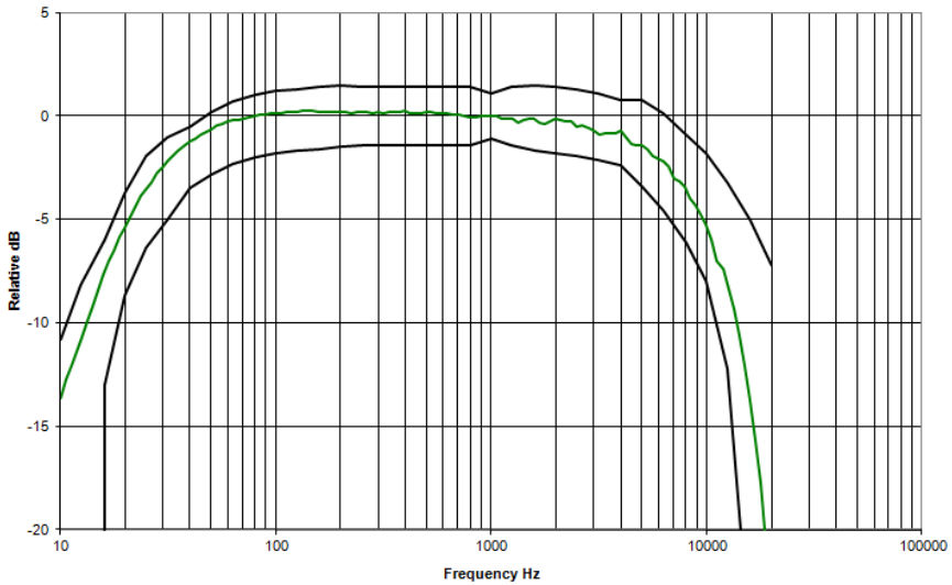
Figure C-6: C-weighting typical
