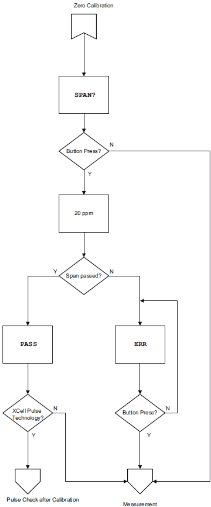
Figure 12 Span calibration
