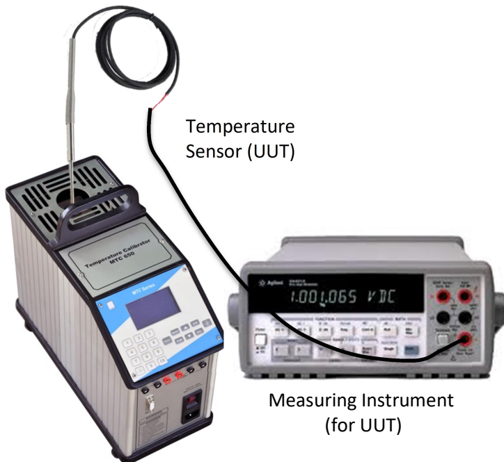
MTC 650 - Universal Dry Block Medium Temperature Calibrator
